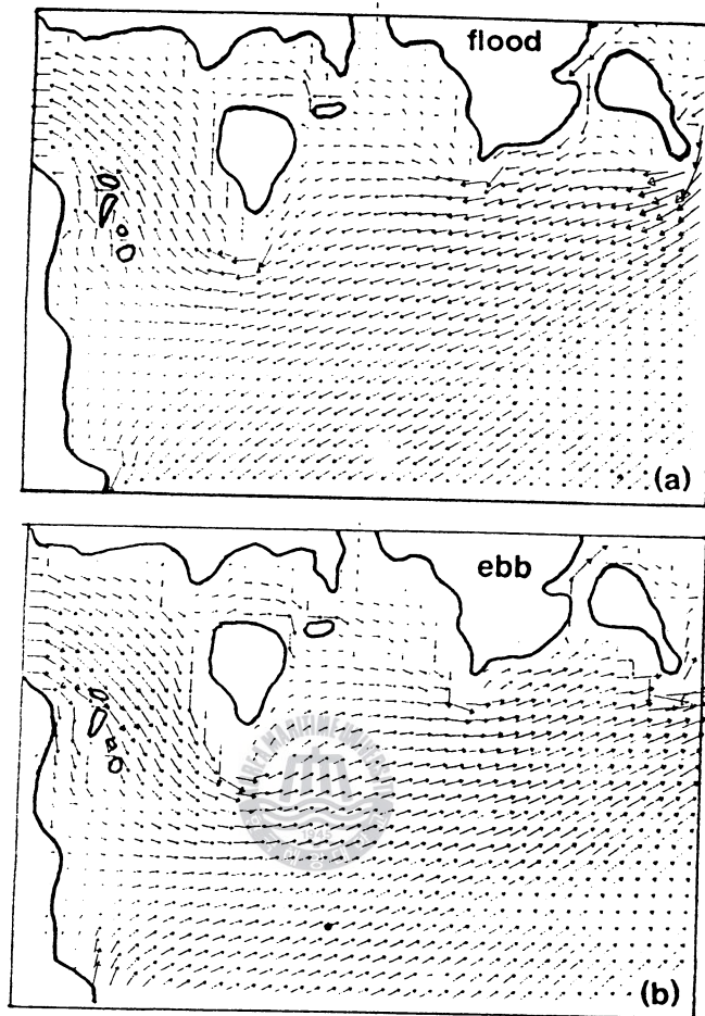
Fig.3 Model boundary and applied flows: (a) flood flow, (b) ebb flow
