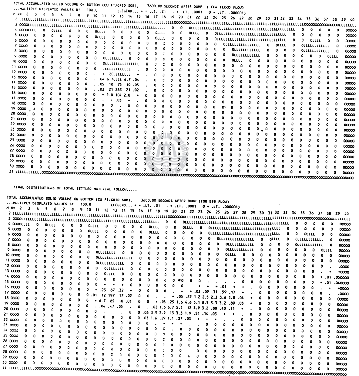
Fig.4 Distribution of deposited solids after 1 hour
