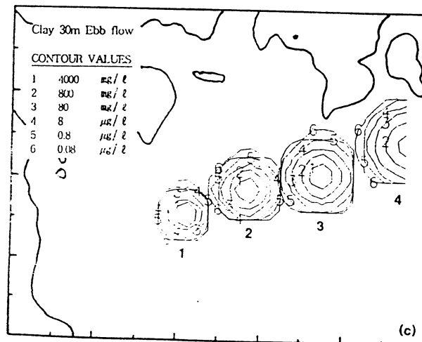
Fig.7 Material distribution for the selected water depth (ebb flow; clay): (a) 3m, (b) 15m, (c) 30m
