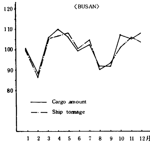
Fig.3-4. Seasonal in of BUSAN between cargo amount and ship's tonnage.
