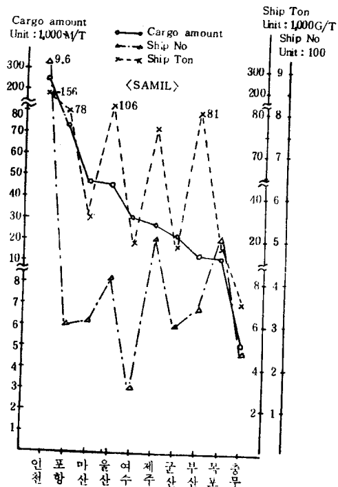
Fig.2-6. Amount of ship's tonnage, numbers and cargoes departing from SAMIL to mainports.
