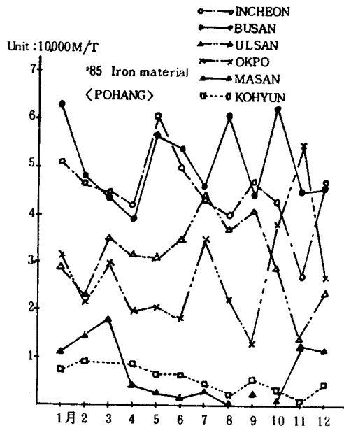
Fig.2-14. Transported amount of iron material from POHANG to mainports per month.
