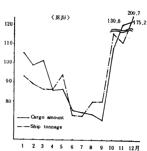
Fig.3-8. Seasonal in of JEJU between cargo amount and ship's tonnage.
