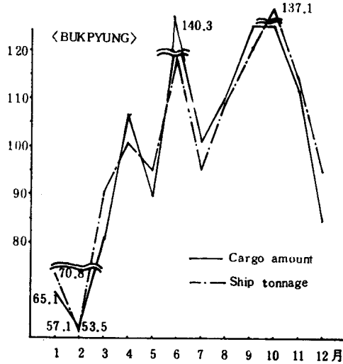
Fig.3-7. Seasonal in of BUKPYUNG between cargo amount and ship's tonnage.
