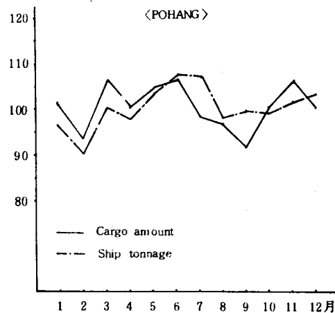
Fig.3-6. Seasonal in of POHANG between cargo amount and ship's tonnage.
