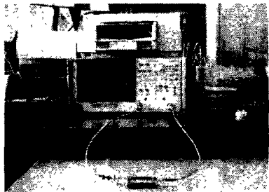
Fig. 5 Set-up to analyze the frequency characteristics of broad-band EMC filter.
