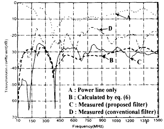
Fig 6 Insertion loss for differential-mode.
