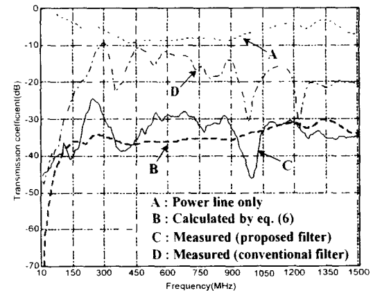
Fig 7 Insertion loss for common-mode.
