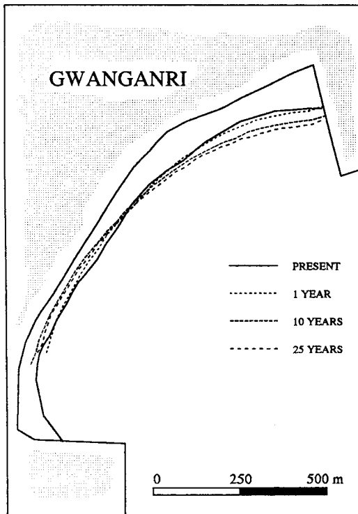
Fig. 6. Shoreline change for the next 25 years at the Gwanganri beach. Solid line (present) represents the average of several field measurements in 1990.
