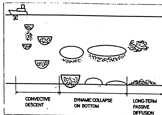
Fig. 2.2 Idealized view of dump of dredged material for development of the numerical model
