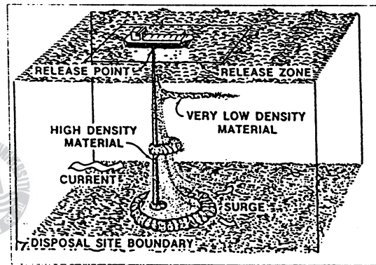
Fig. 2.1 Overview of deposition process from the barge
