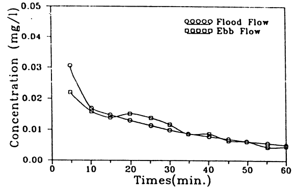
Fig. 5.2 Change of peak contaminant concentration in water column with respect to time
