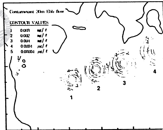
Fig. 5.6 Contaminant distribution for 30m water depth with respect to time(ebb flow)
