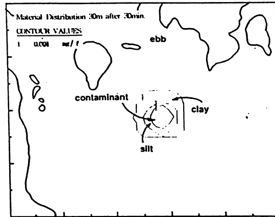
Fig. 5.5 Material distribution for 30m water depth(ebb flow)
