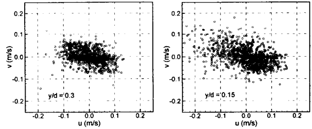
Fig. 7 Sample outputs of fluctuating velocities u'v' .
