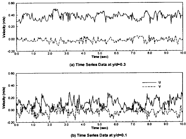
Fig. 5 Typical time-series data converted from PIV data.
