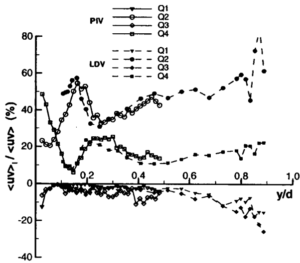
Fig. 8 Quadrant analysis for X/h=4 .
