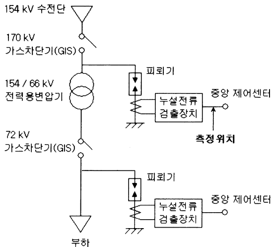
Fig. 1 Measuring point of surges
