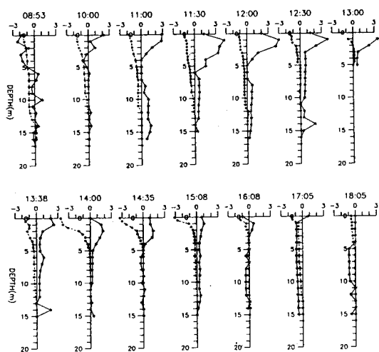
Fig. 3. Vertical distribution of currents in north-south direction (solid line, scale × 10 cm/sec) and the salinity difference at each depth from the bottom (broken line, scale × 1%).
