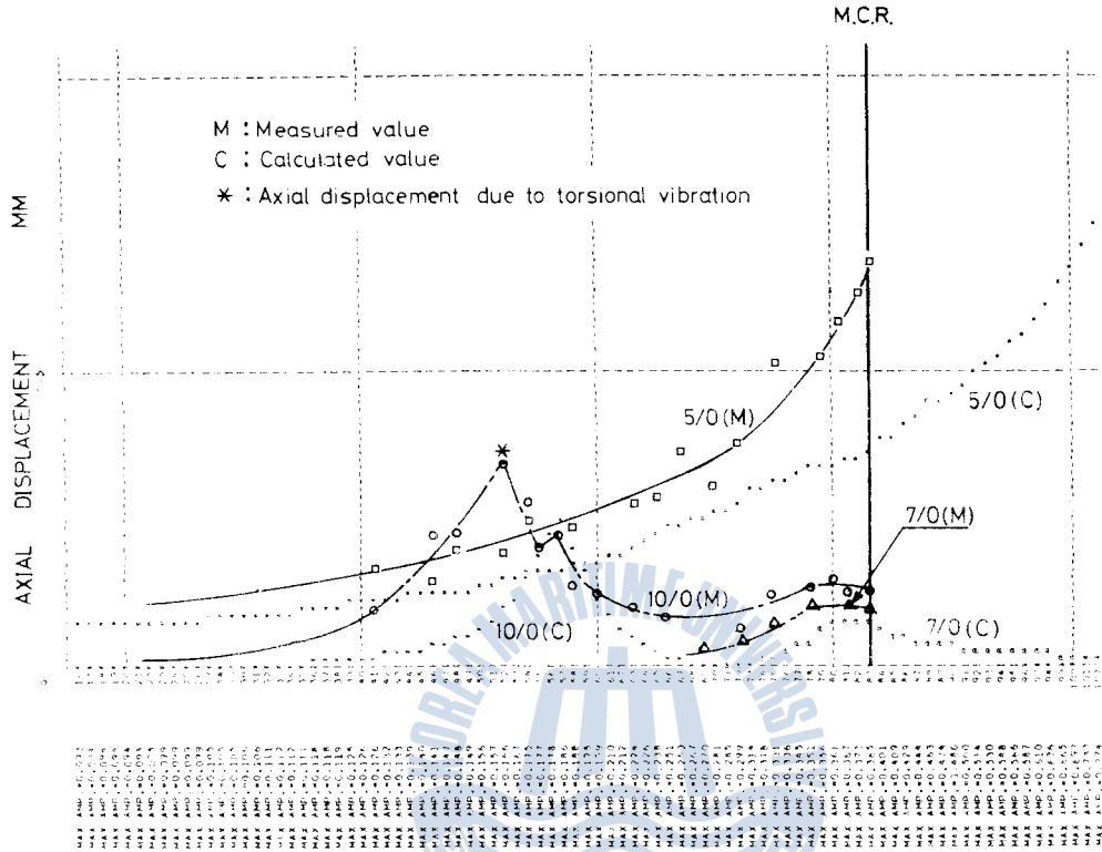
Fig. 4 Displacement of axial vibration at crankshaft fore-end(5L80MCE)
