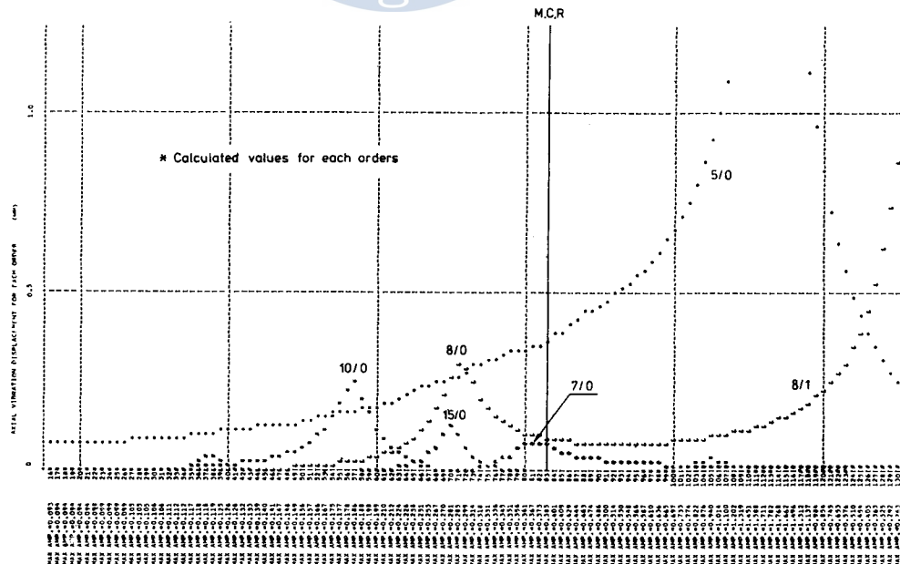
Fig. 3 Displacement of axial vibration for each order (5L80MCE)
