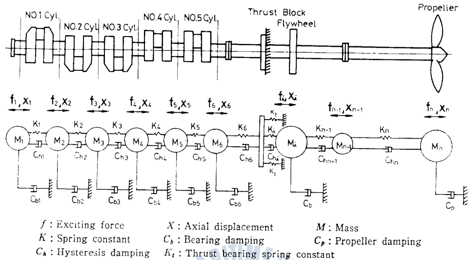
Fig. 1 Axial vibration system for marine diesel engine propulsion shafting
