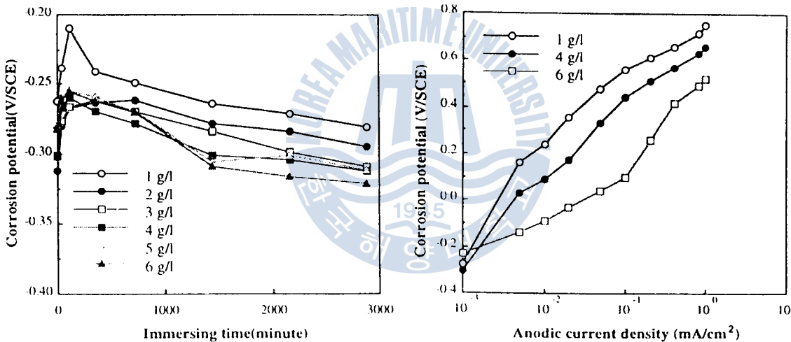
Fig.5 Variation of corrosion potential according to NaOH addition as a function immersed time in 3% NaCl solution
