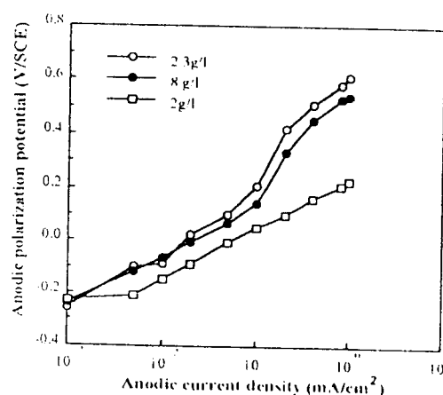
Fig.9 Variation of anodic polarization curves as a function of Glycine addition in 3% NaCl solution
