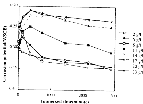
Fig.8 Variation of corrosion potential according to Glycine addition as a function immersed time in 3% NaCl solution
