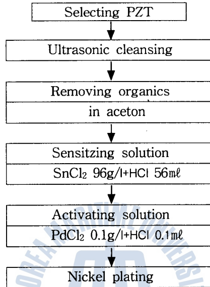
Fig. 1 Process of Electroless Nickel plating
