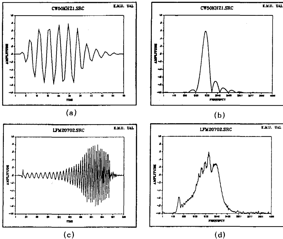
Fig.4 Source signal (a) CW source signal (b) spectrum of CW source signal (c) FM source signal (d) spectrum of FM source signal
