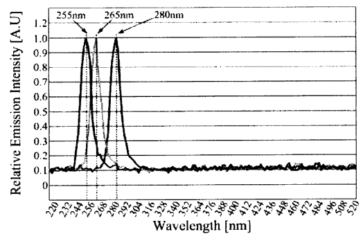
Fig. 4 Spectrum of the UV LED modules
