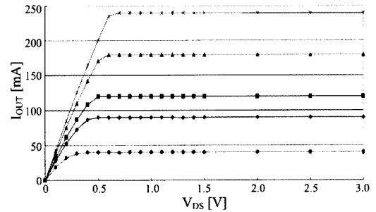
Fig. 3 Current characteristics of the fabricated LED driver
