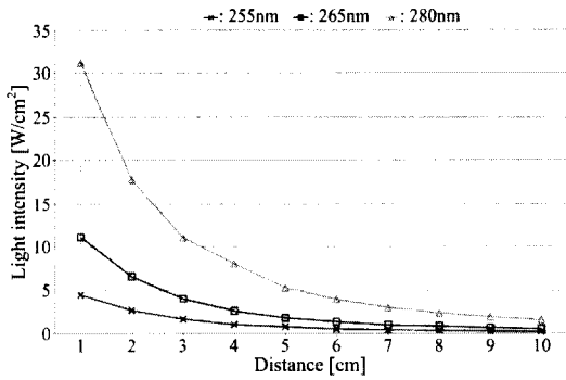
Fig. 5 Intensity of the UV LED modules
