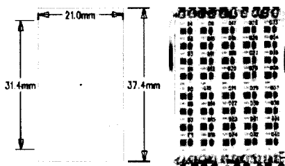
Fig. 1 Configuration of the UV LED module
